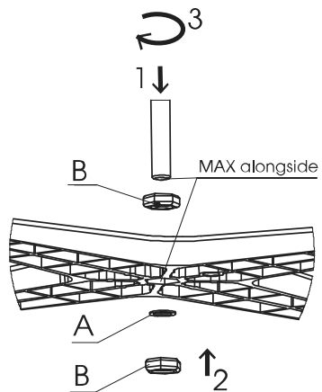
DETAIL 1
