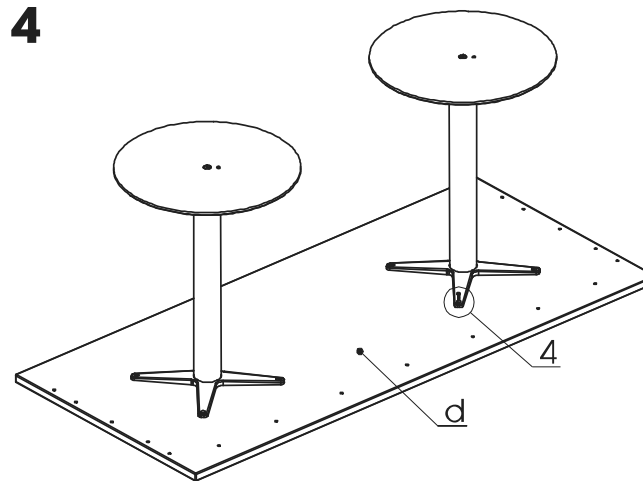
DETAIL 4
