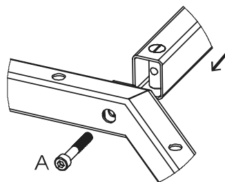
DETAIL 2.2
