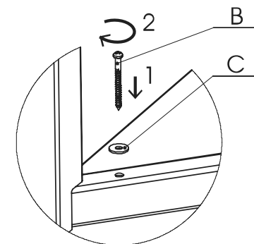
DETAIL 4
